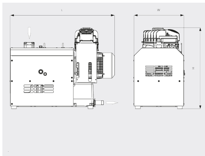
Dimensional drawing
