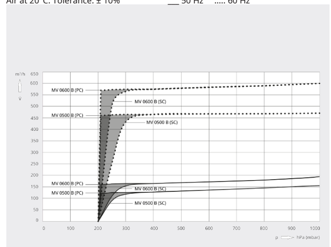
Pumping speed
