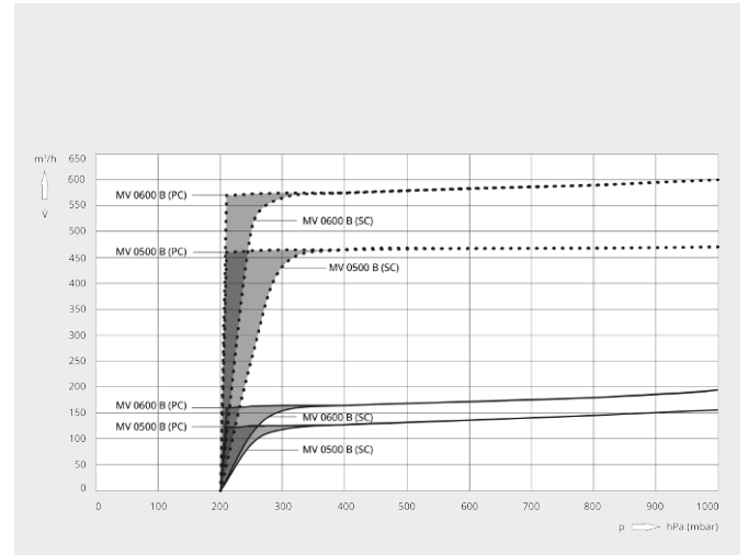
Pumping speed
