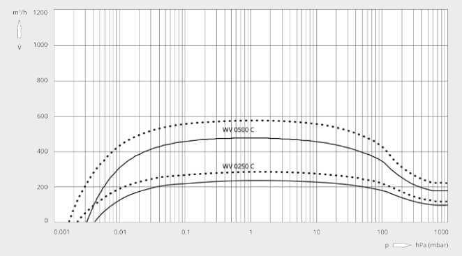
Pumping speed
