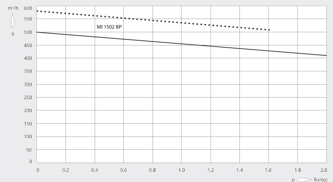
Pumping speed
