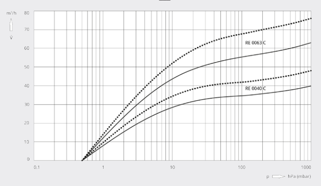
Pumping speed
