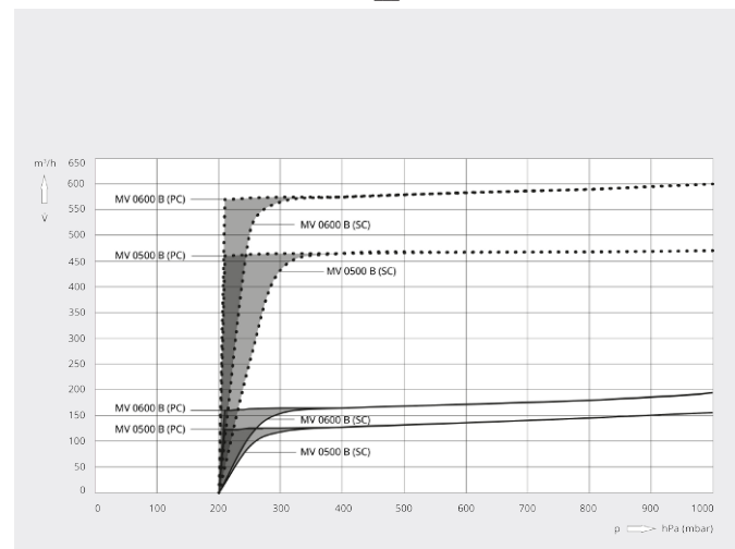
Pumping speed
