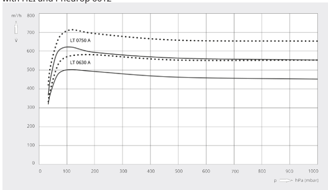
Pumping speed
